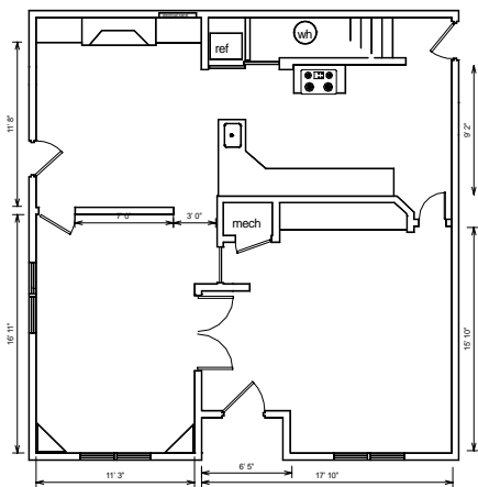
1 1 Plan Ground Floor SCALE 1/4" = 1'-0"
