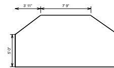
3 1 Section Second Floor SCALE 1/4" = 1'-0"
