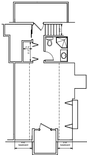
2 1 Plan Second Floor SCALE 1/4" = 1'-0"
